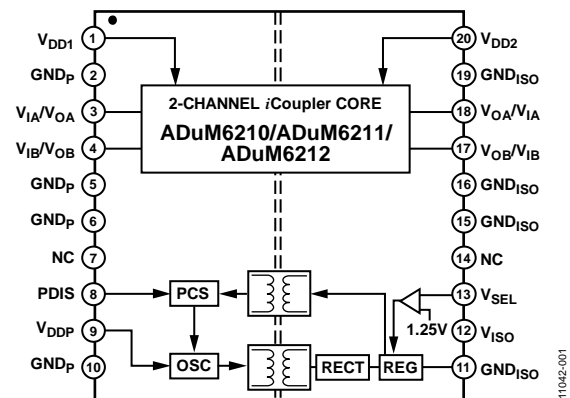
Figure 1. ADuM6210/ADuM6211/ADuM6212
