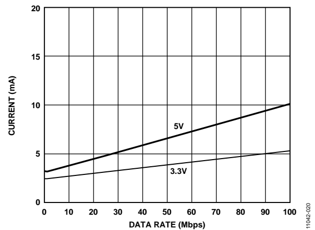
Figure 22. Typical ADuM6210 V_{DD2} or ADuM5212 V_{DD2} Supply Current vs. Data Rate for 5 V and 3.3 V Operation
