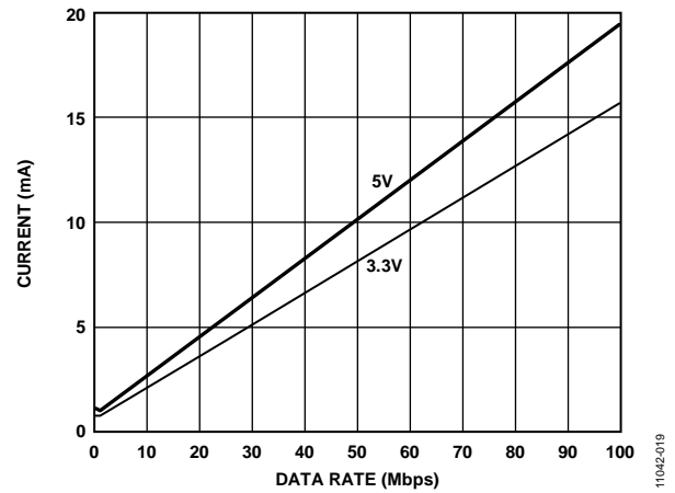
Figure 21. Typical ADuM6210 V_{DD1} or ADuM5212 V_{DD2} Supply Current vs. Data Rate for 5 V and 3.3 V Operation
